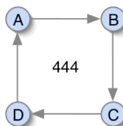
Figure 3. Possible graphs from 2, 3 and 4 edges. Edges can be either unidirectional or bidirectional (bidirectional edges are counted as two edges).
